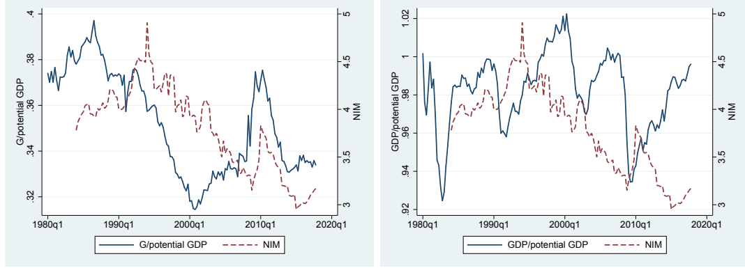
Figure 1: Cyclicity of Spreads
