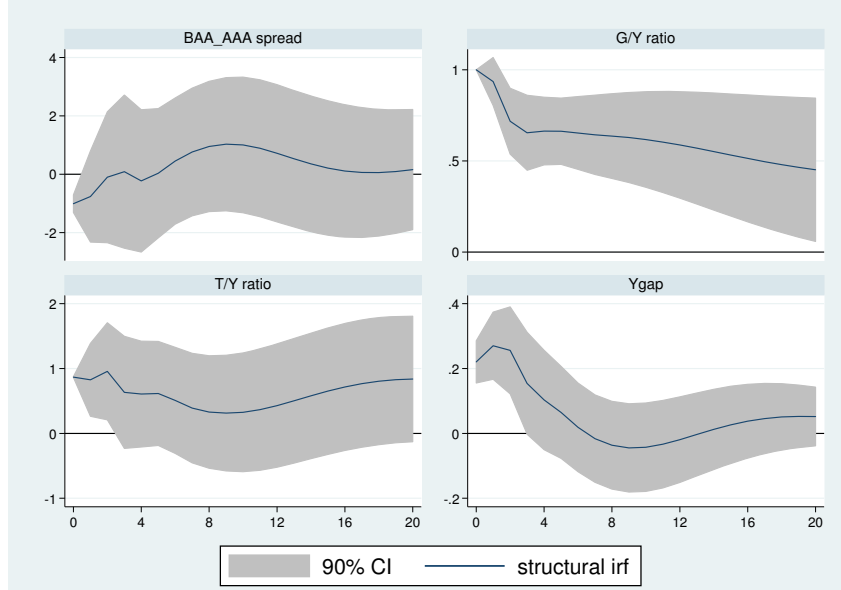
Figure 4: Impulse response functions to a 1% increase in \frac{G}{Y} ratio when spread = Baa-Aaa.
