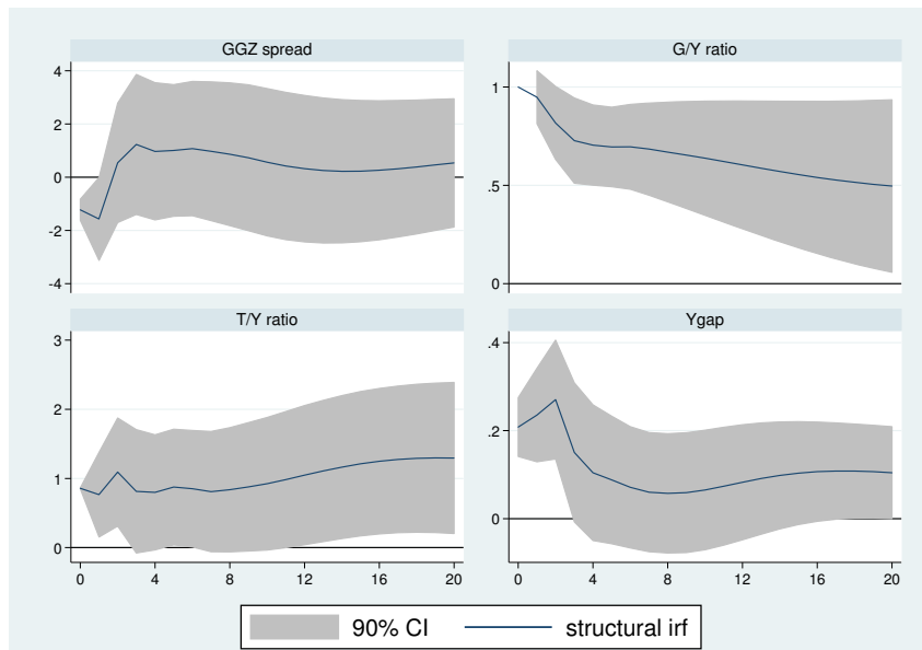
Figure 3: Impulse response functions to a 1% increase in \frac{G}{Y} ratio when spread = GGZ.
