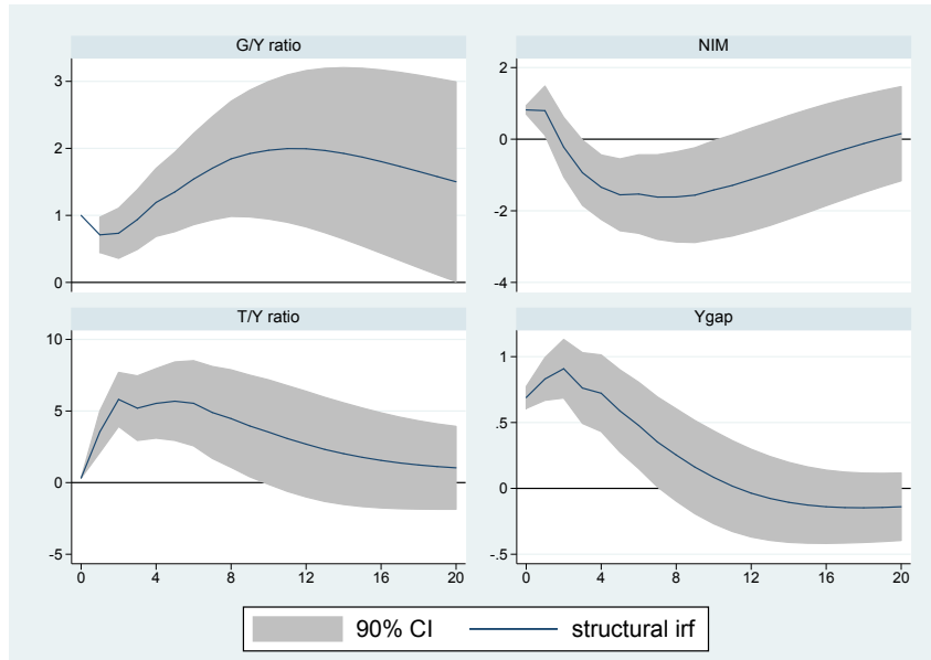
Figure 2: Impulse response functions to a 1% increase in \frac{G}{Y} ratio when spread = NIM.
