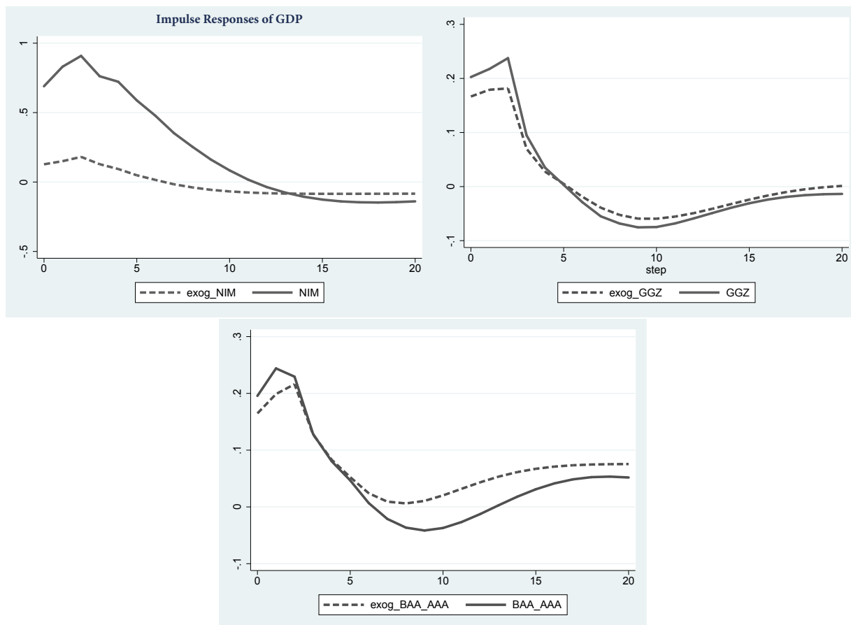
Figure 5: Impulse response functions for GDP - Comparison to case of exogenous spreads.
