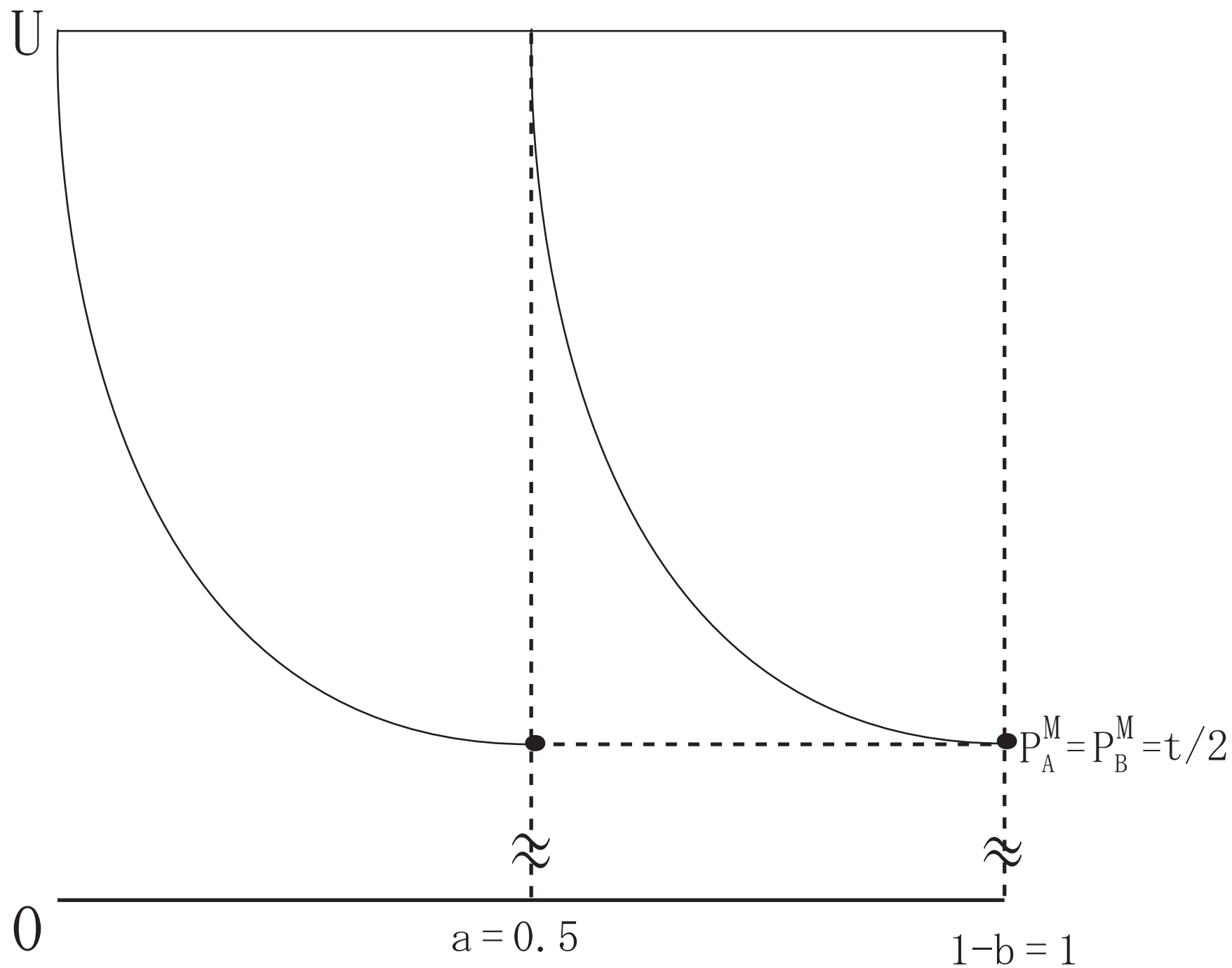
Figure 1: The case where U/t = 3/4
