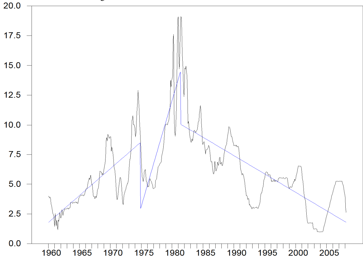
Figure 1: The FFR series with two trend breaks
