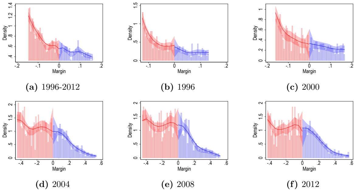
Figure 1: Manipulation testing plots
